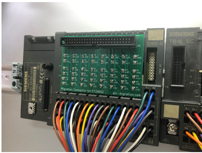
terminal block "TB 16 IM-SC" and migration connector
